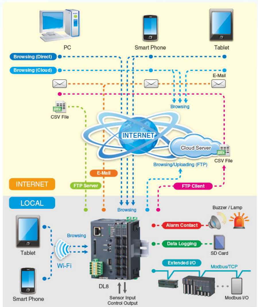
Web-Enabled Remote Terminal Unit for Monitoring, Event Reporting and Data Logging Model: DL8
